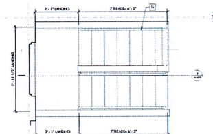
1 STAIR PLAN
