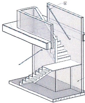
3 STAIR AXON
