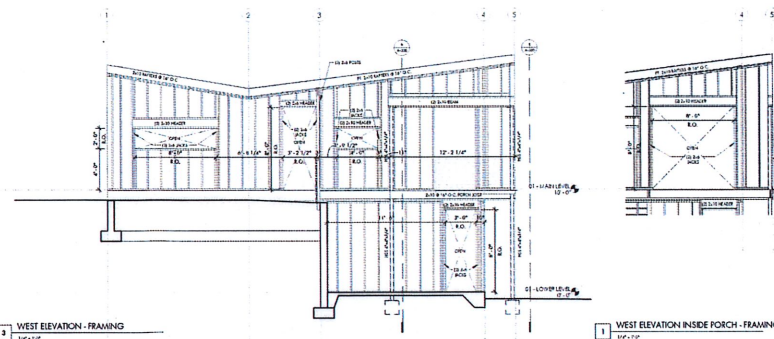
1 WEST ELEVATION INSIDE PORCH - FRAMING MC-10P
