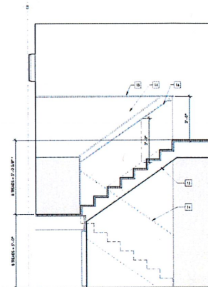
2 STAIR SECTION
