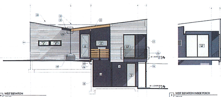
2 WEST ELEVATION INSIDE PORCH
