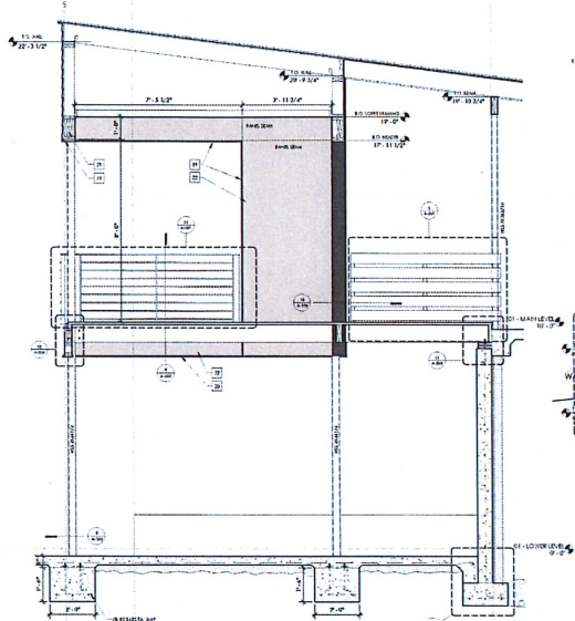
2 WALL SECTION @ COLUMN 'B'
